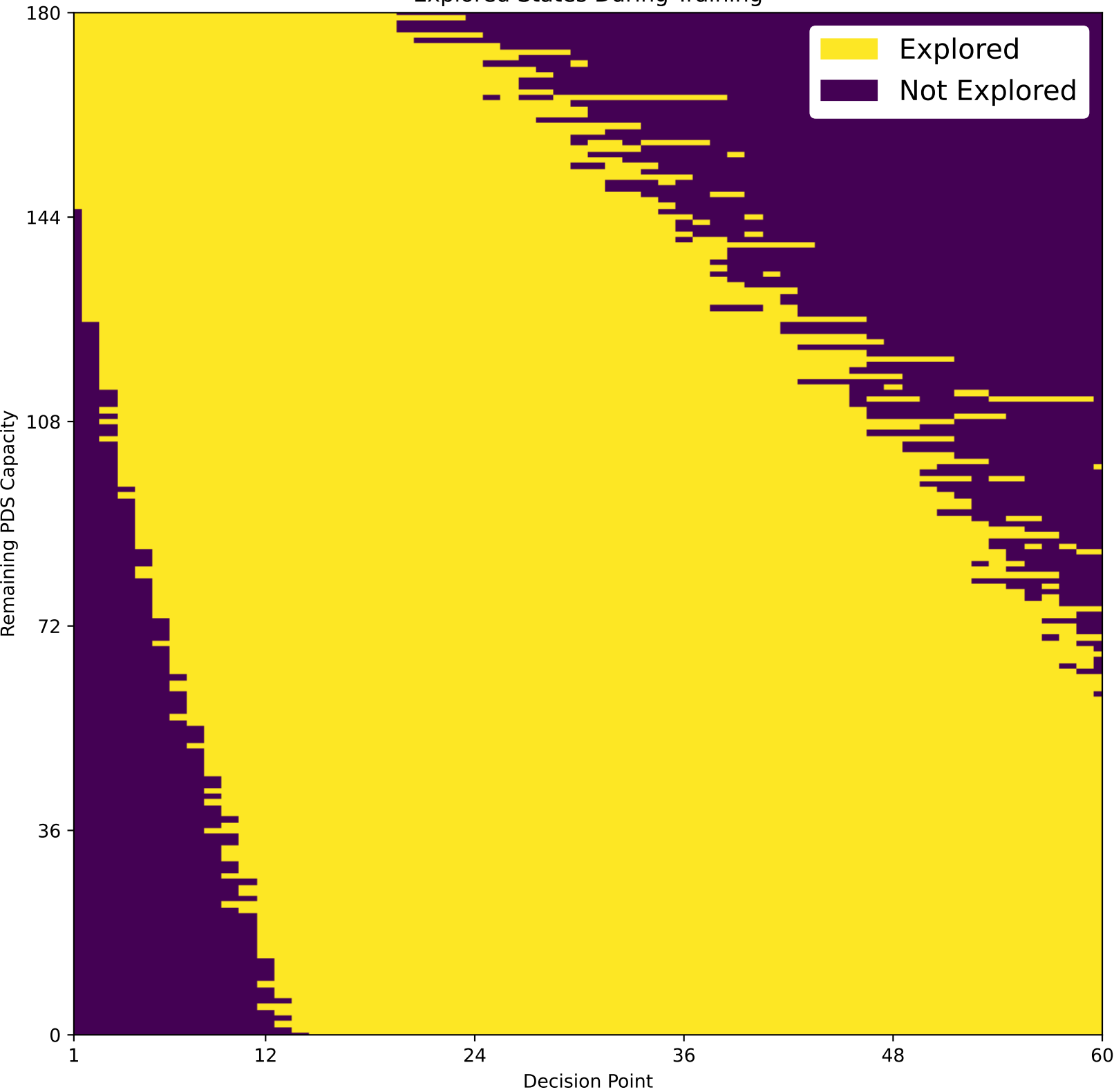
Explored States During Training
